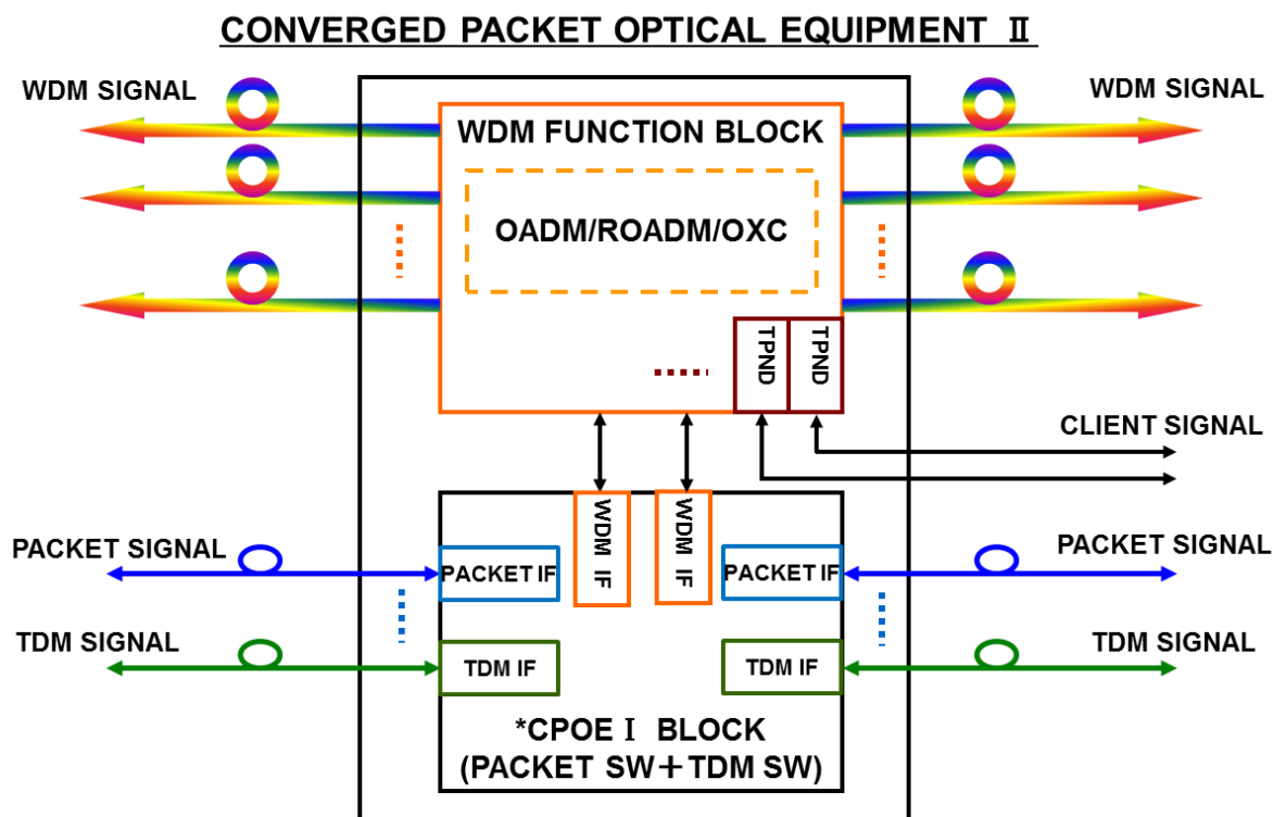
*CPOE I : CONVERGED PACKET OPTICAL EQUIPMENT I
