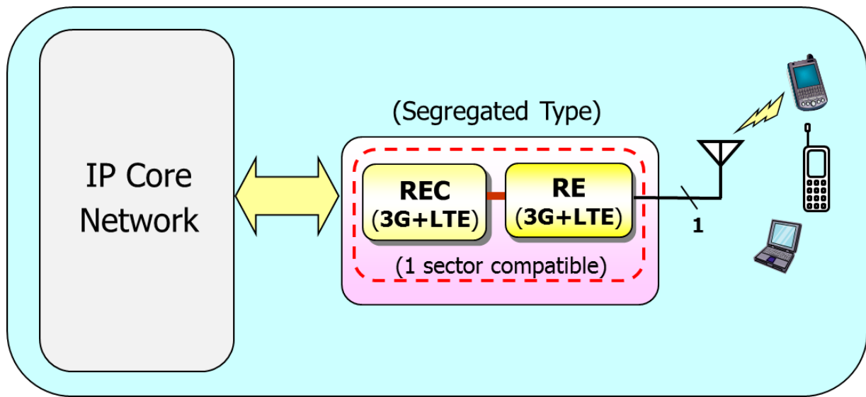
Scope of 3G and LTE multi-standard Radio Base Station Equipment
