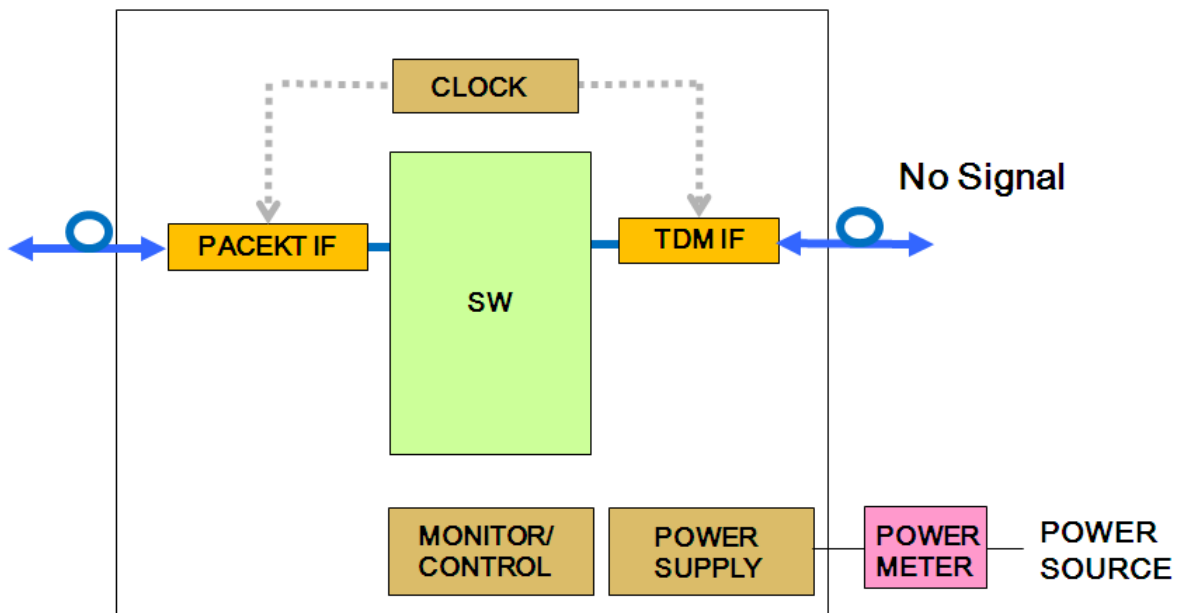
[Example of minimum component and path configuration for measuring P_{idle} ]
